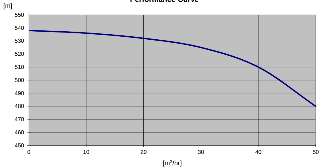
Performance Curve
